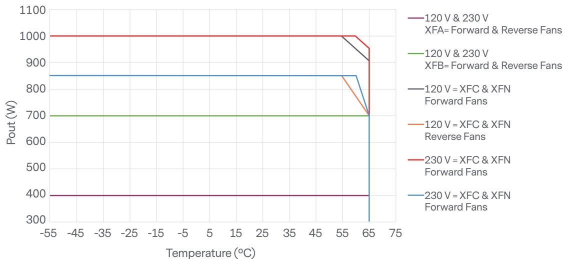
Temperature Derating Curve for XF Models
