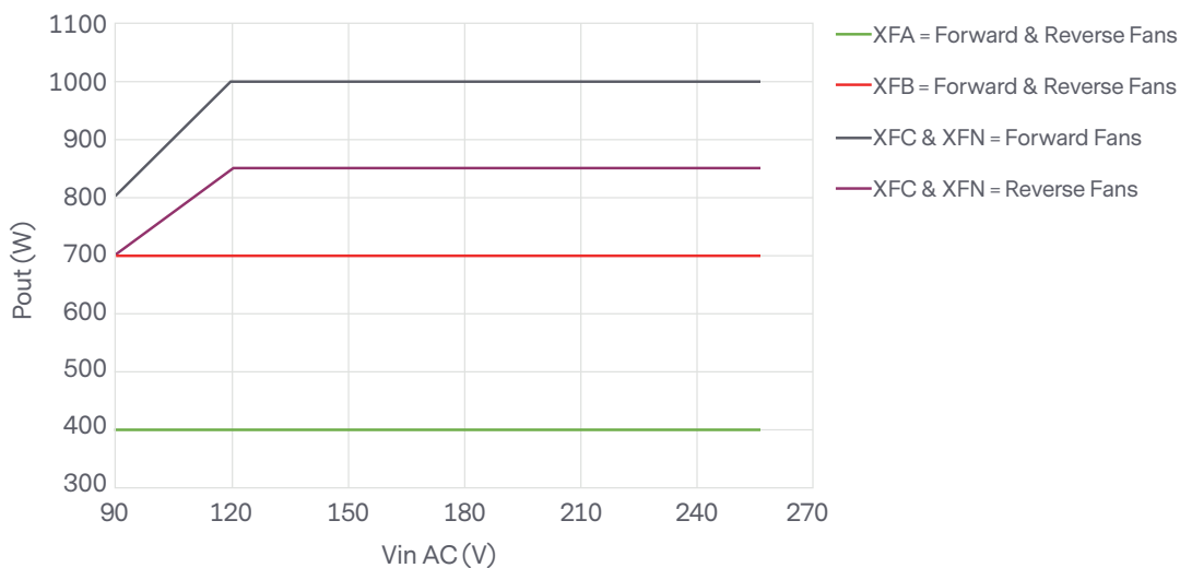
Line Derating Curve for XF Models (@ 60°C)
