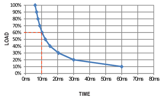
RSD-60G-24
