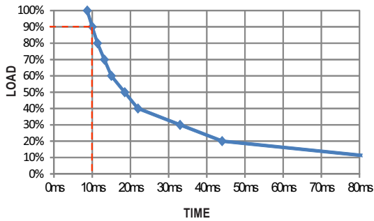
RSD-60G-3.3
