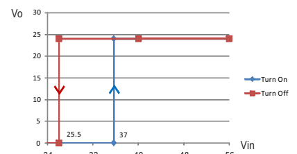
RSD-60H-24
