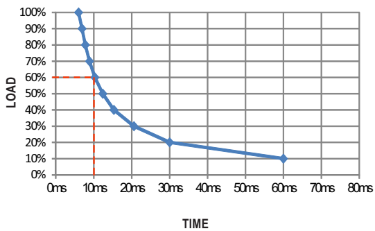
RSD-60G-12
