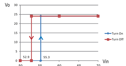
RSD-150D-24
