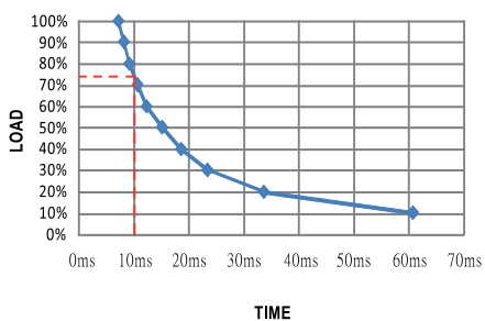
RSD-150C-5
