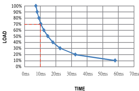
RSD-150C-12
