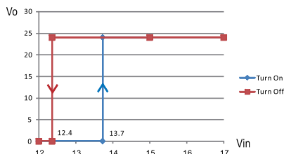
RSD-150B-24
