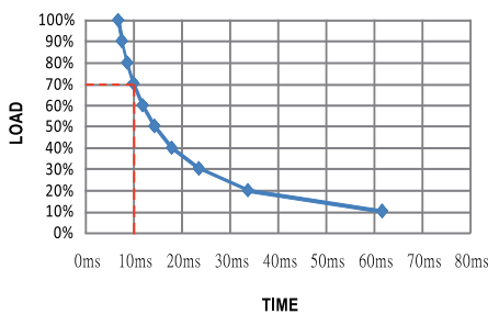
RSD-150C-12
