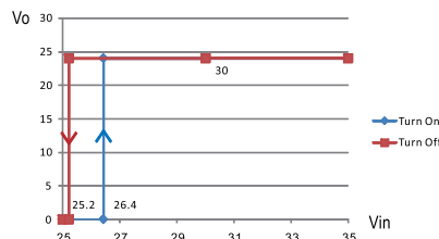
RSD-150C-24
