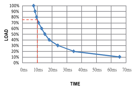
RSD-150C-24
