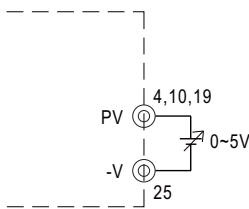
Fig. 2.1 Add on 0~5V external voltage
