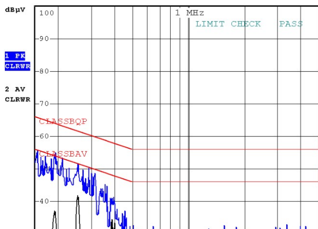
Typical phase conducted emission at 230 V AC , 50 Hz
