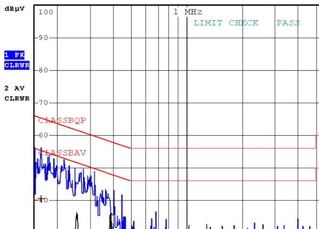
Typical phase conducted emissions at 120 V AC , 60 Hz
