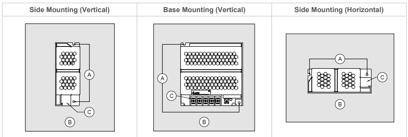
Fig. 2 Mounting Orientation
