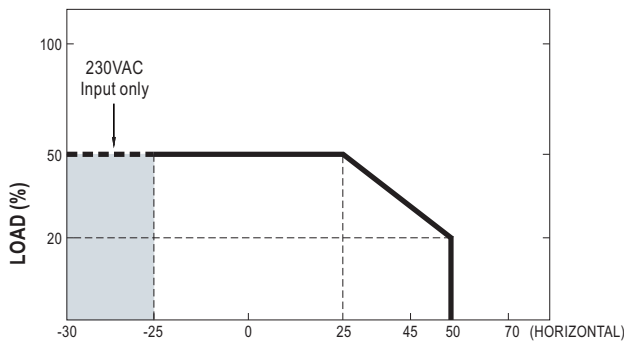
AMBIENT TEMPERATURE WITHOUT ALUMINUM PLATE(°C)
