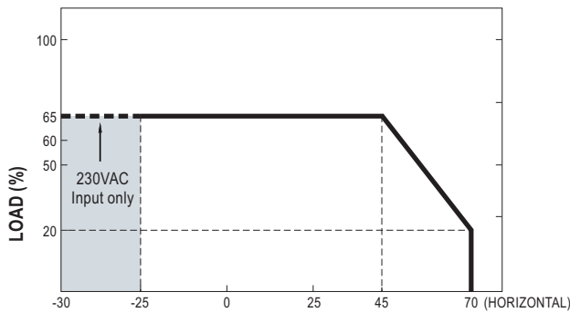
AMBIENT TEMPERATURE WITH ADDITIONAL ALUMINUM PLATE(°C) (450x450x3mm)
