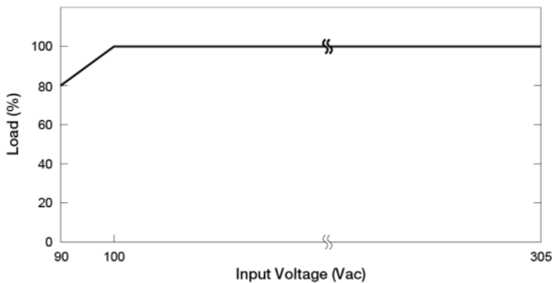
Fig. 2 De-rating for Low Input Voltage (All Models)
