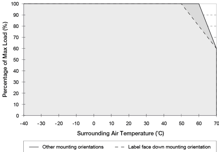
Fig. 1 De-rating for Label face down mounting orientation
