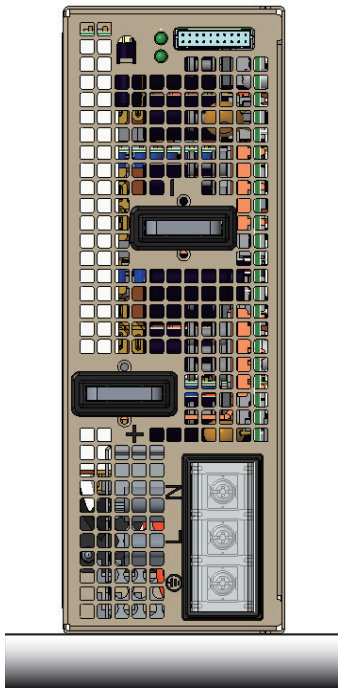
MOUNTING "A"
