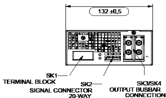
PSU Front View (24V & 48V UNITS)
