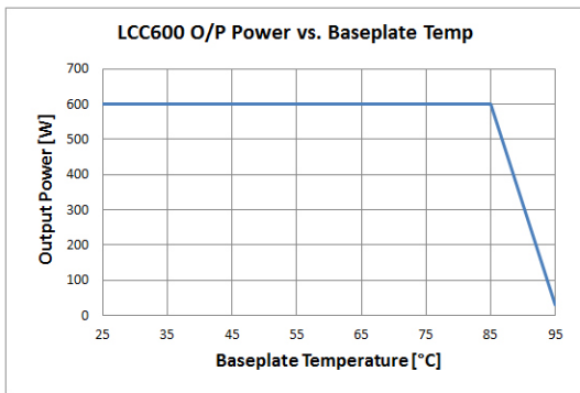
Figure 1. Output Power vs. Baseplate Temperature
