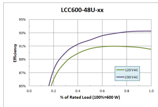
Figure 4. Typical Efficiency for 48 V output
