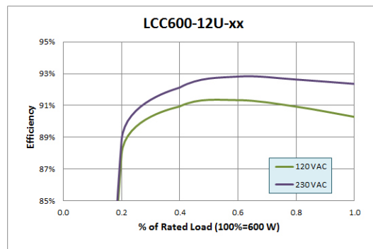
Figure 6. Typical Efficiency for 12 V output
