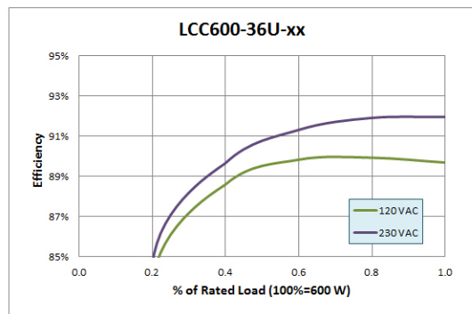
Figure 5. Typical Efficiency for 36 V output
