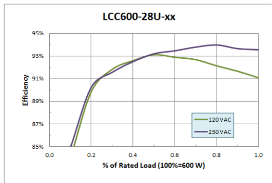
Figure 3. Typical Efficiency for 28 V output
