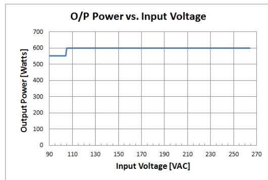
Figure 2. Output Power vs. Input Voltage
