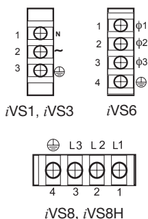
Figure 1. AC Input
