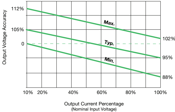
Fig 3. 5/9/12/15/24VDC Output
