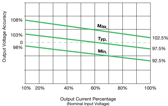
Fig 3. 5/9/12/15/24VDC Output
