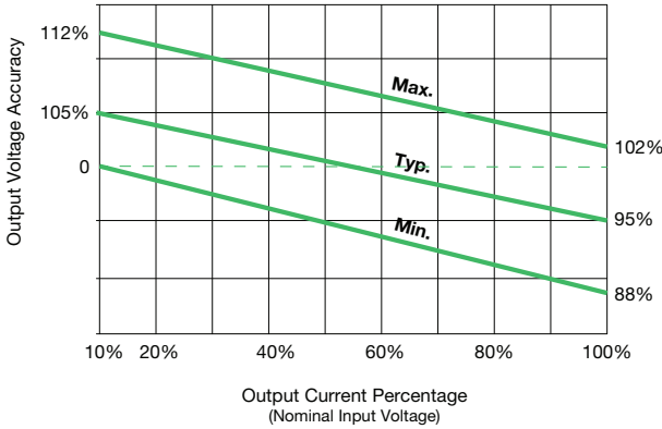
Fig 3. 5/9/12/15/24VDC Output
