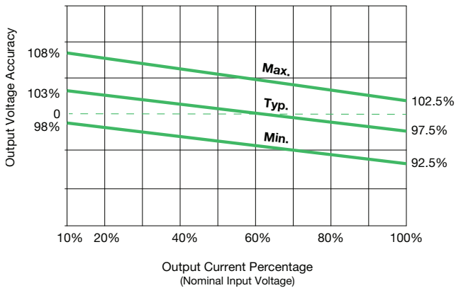
Fig 3. 5/9/12/15/24VDC Output
