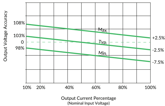
Fig 3. 5/12/15/24VDC Output
