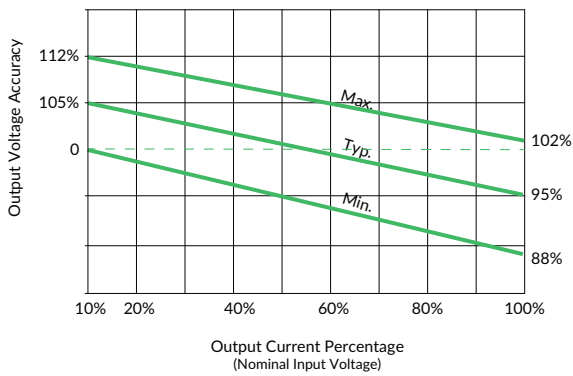
Fig 3. 5/12/15/24VDC Output
