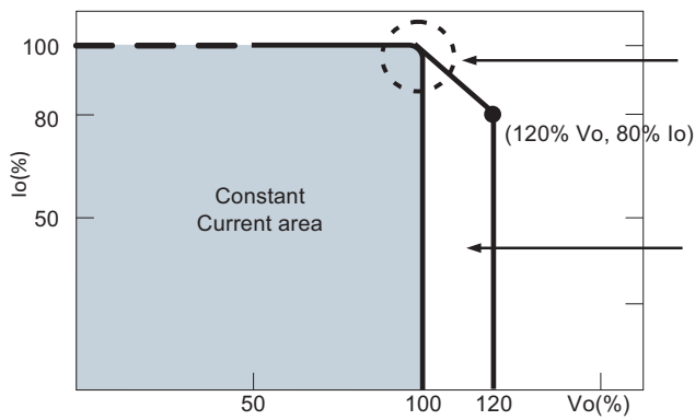
Typical LED driver I-V curve
