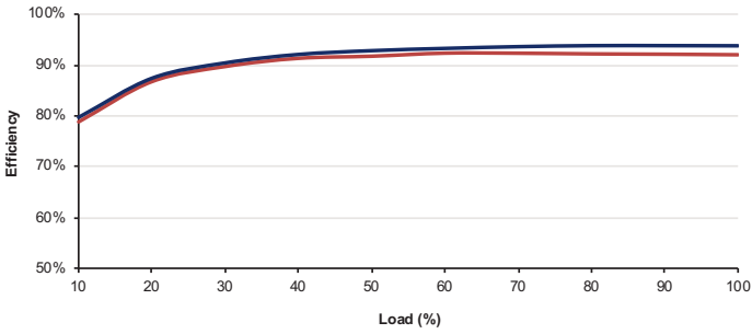
Figure 1 - ECH450PS12 (250W)
