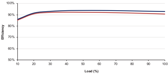
Figure 3 - ECH450PS24 (250W)
