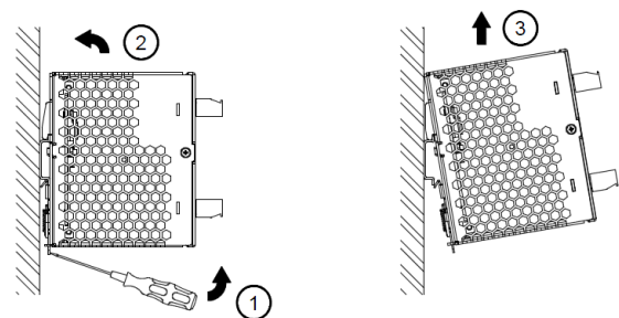
Fig. 2.2 Dismounting
