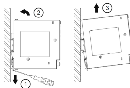
Fig. 6.2 Dismounting
