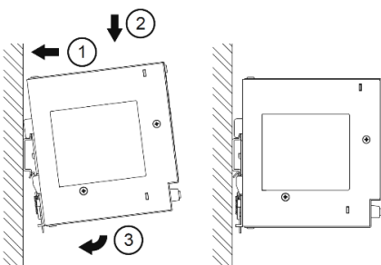
Fig. 6.1 Mounting
