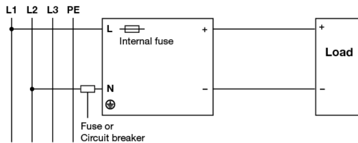
Fig. 13 2 of 3 Phase System Input Operation Connection Diagram
