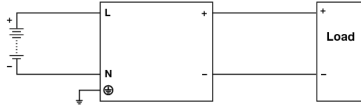
Fig. 12 DC Input Operation Connection Diagram
