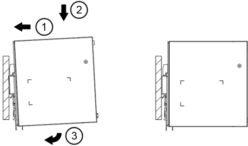
Fig. 3.1 Mounting
