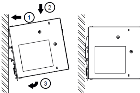
Fig. 3.1 Mounting
