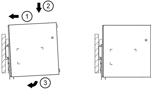
Fig. 3.1 Mounting
