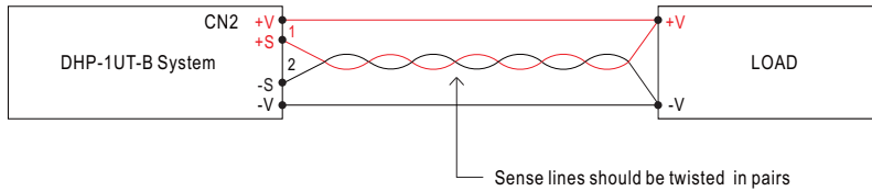
Figure 1-1 Connection of Remote Sense
