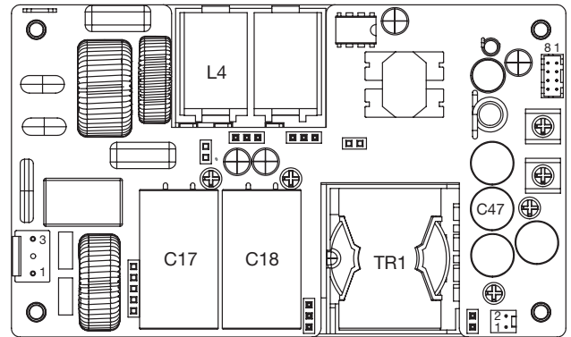
Upper PCB
