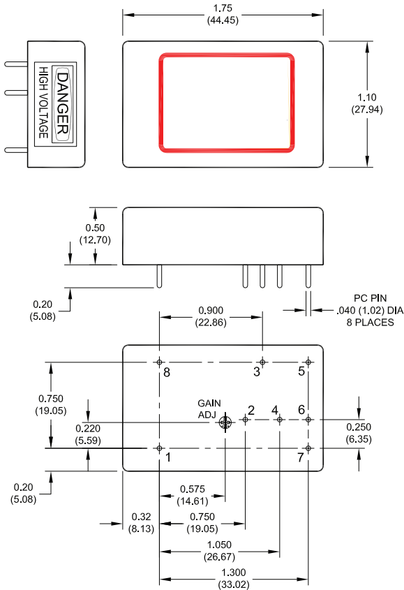
Top View
