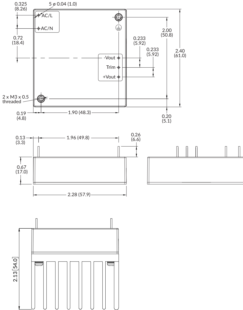
Optional version with heat-sink fitted.
