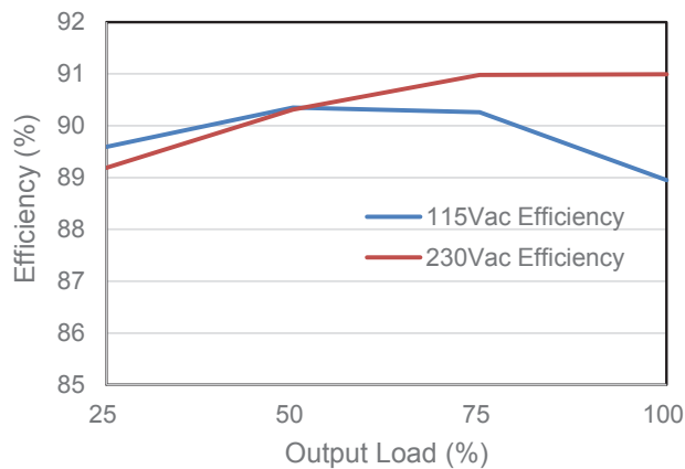
Figure 1-3 MEA-065A19C Efficiency versus Output Load
