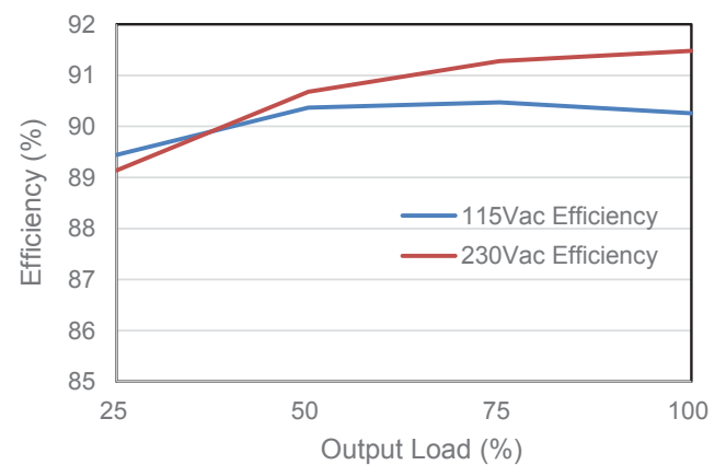
Figure 1-4 MEA-065A24C Efficiency versus Output Load
