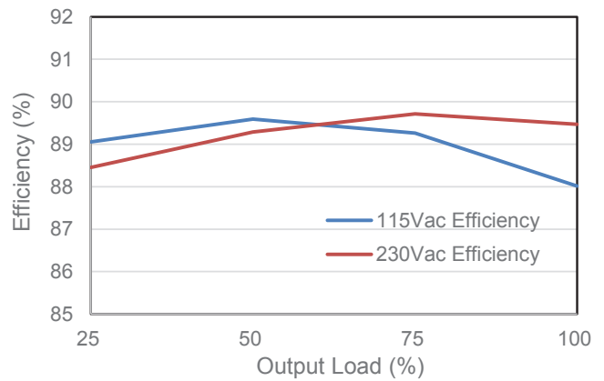
Figure 1-2 MEA-065A15C Efficiency versus Output Load
