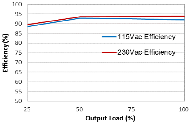
Fig.1-3 MDS-400AUS30 BA Efficiency versus output load
