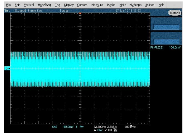
Fig. 2 Ripple & Noise example, 20 MHz BW
