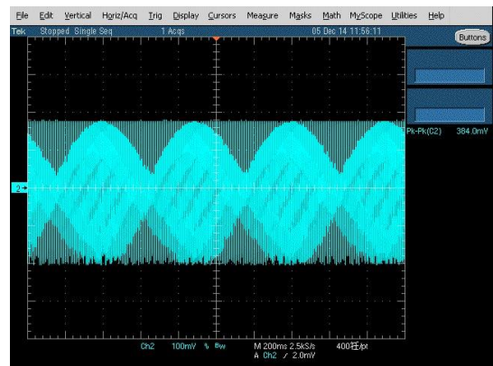
(b) 230 V (measured value=384 mV)
