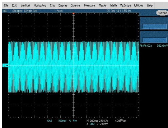
(a) 115 V (measured value=392 mV)
