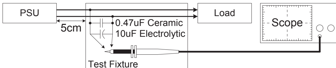
Fig. 3 Ripple & Noise measurement circuit
