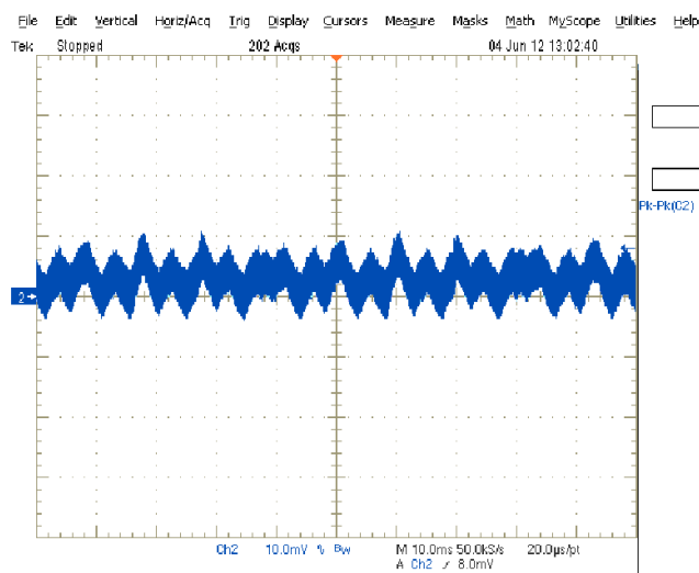
(a) 115 V
