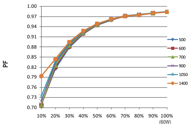
LOAD (230Vac Input)
