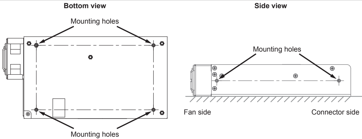
Fig. 5: Position of the mounting holes
