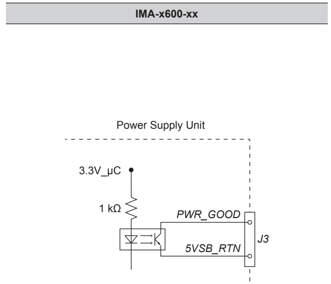
Fig. 20: Circuit diagram J3 Pin 9 (PWR_GOOD)
