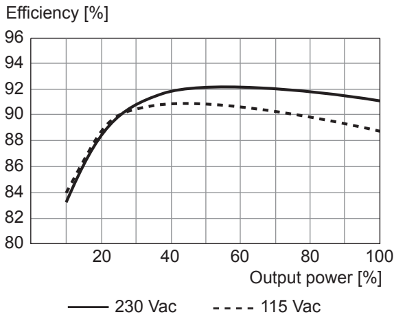
Fig. 15: Typical efficiency curves 12 V
