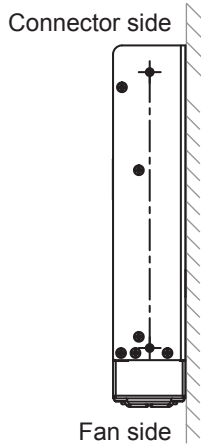
Fig. 2: Vertical mounting
