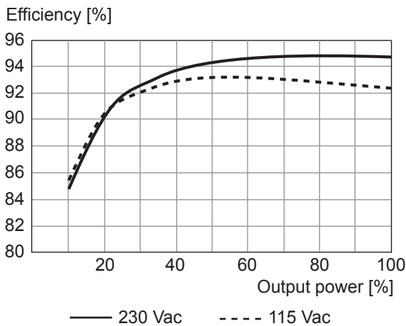
Fig. 17: Typical efficiency curves 48 V
