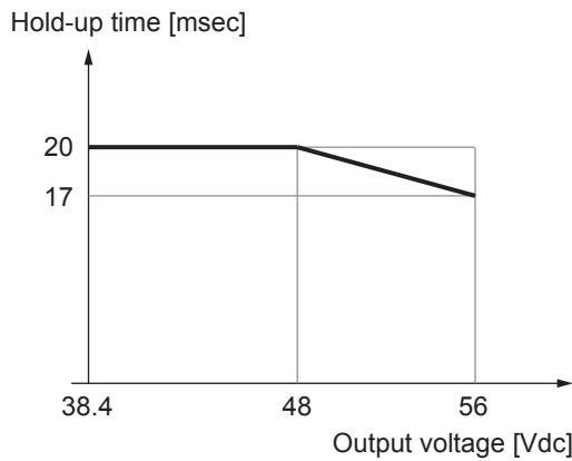
Fig. 15: Hold-up time versus output voltage 48 V
