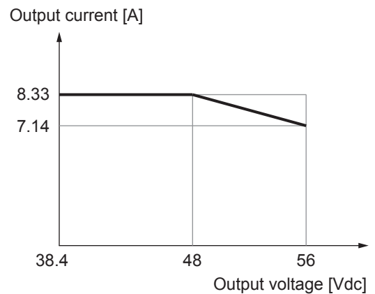
Fig. 12: Output current versus output voltage 48 V
