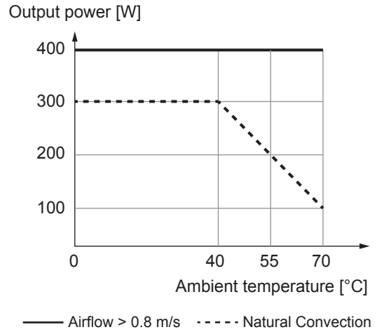
Fig. 8: Output power versus ambient temperature 24/48 V
