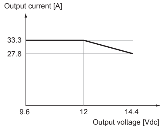
Fig. 10: Output current versus output voltage 12 V
