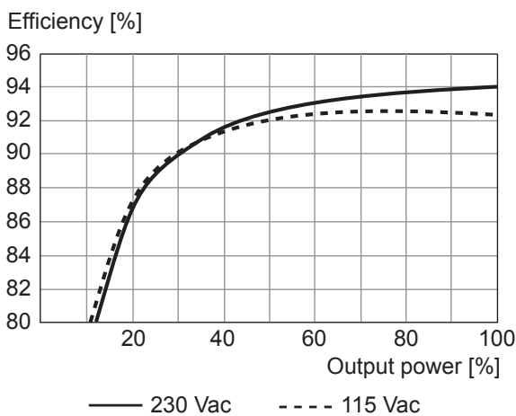
Fig. 17: Typical efficiency curves 24 V
