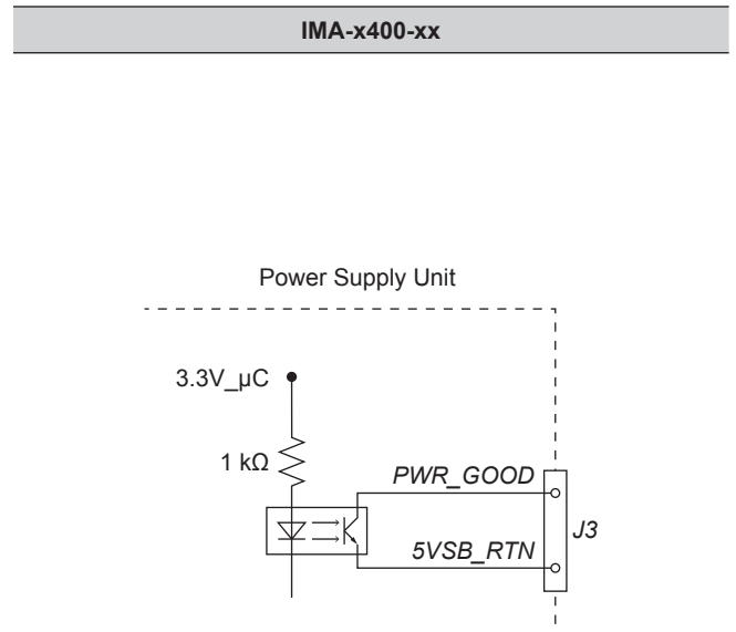
Fig. 21: Circuit diagram J3 Pin 9 (PWR_GOOD)
