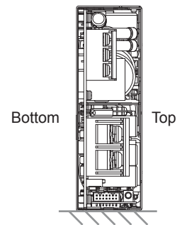
Fig. 4: Mounting on the right side
