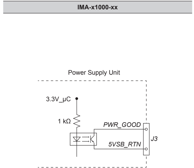
Fig. 17: Circuit diagram J3 Pin 9 (PWR_GOOD)
