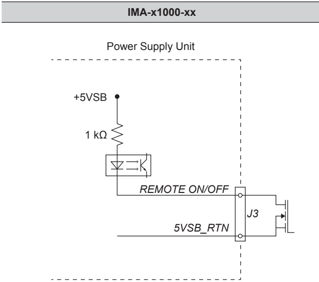
Fig. 16: Circuit diagram J3 Pin 10 (REMOTE ON/OFF)
