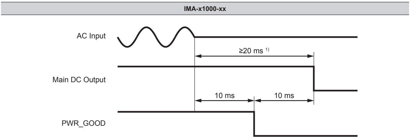
Fig. 18: Power Good function Timing
